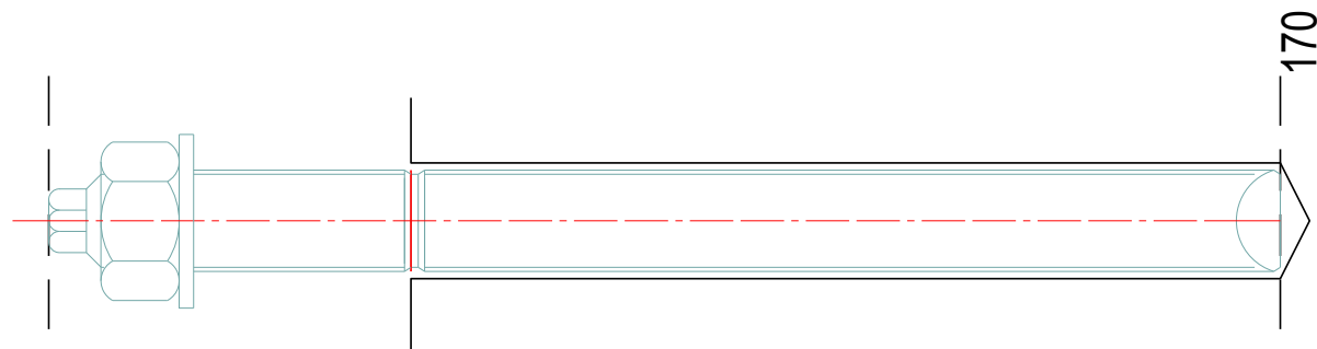
PROFIX PASTA-R M14 x 170
